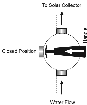
Water flow to Solar Collector
